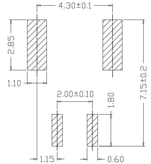
PCB LAYOUT
